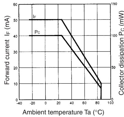
Forward Current vs. Collector Dissipation Temperature Rating
