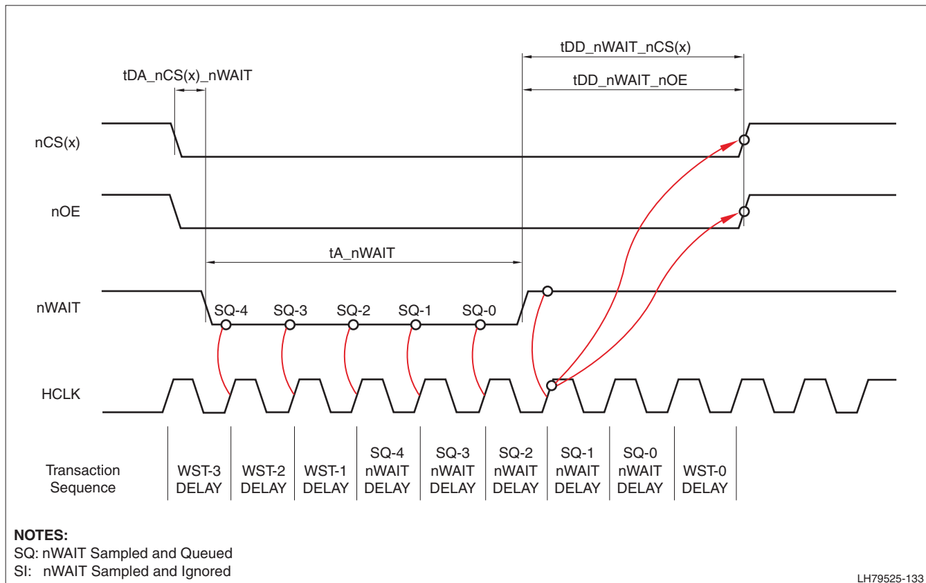
Figure 9. nWAIT Read Sequence (SWAITRDx = 3)
