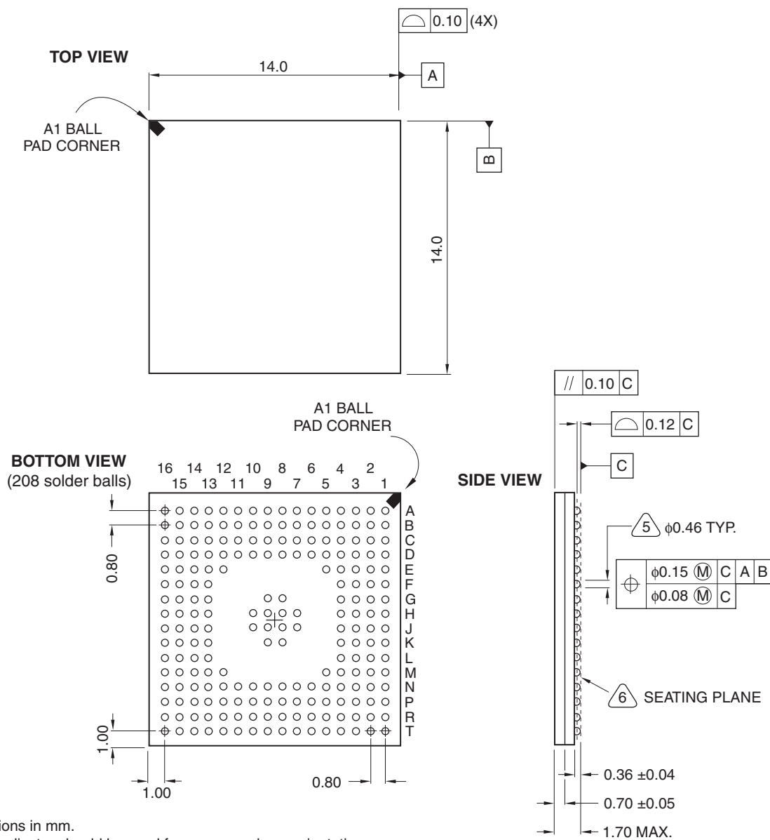
Figure 40. LH79524: 208-ball CABGA
