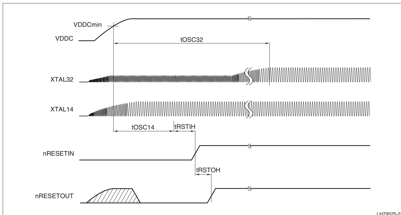
Figure 35. PLL Start-up
