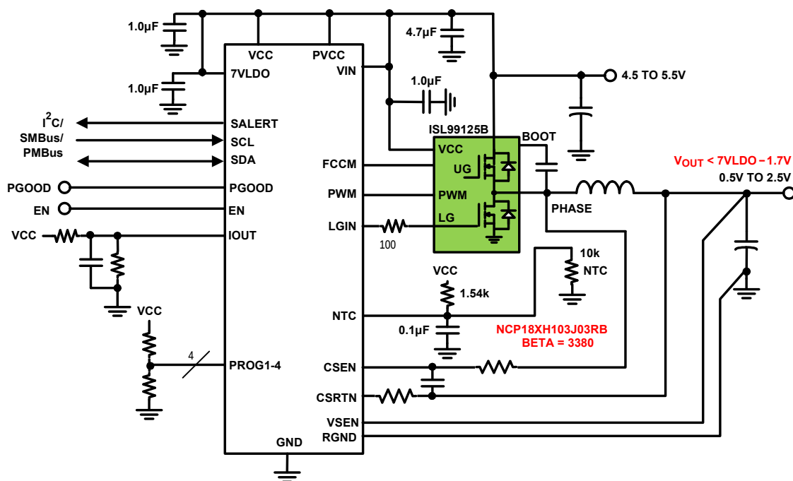
FIGURE 4. 5V INPUT APPLICATION
