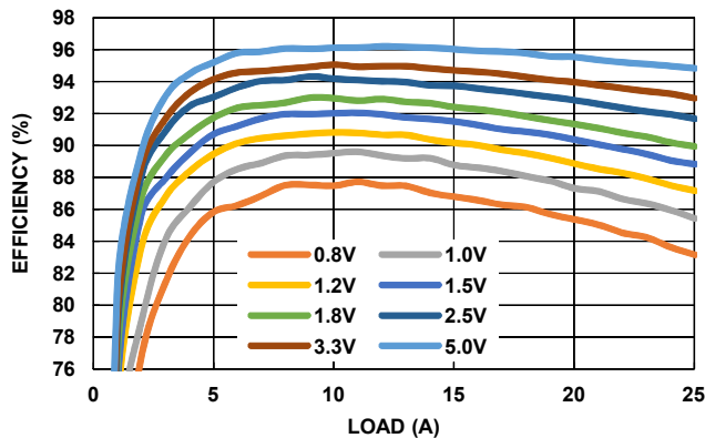
FIGURE 13. POWER STAGE EFFICIENCY ( V_{IN} = 12V ; 400kHz L_{OUT} = 0.47\mu H/0.32m\Omega /WE 744-301-047; INCLUDE INDUCTOR AND ISL99125B LOSSES)
