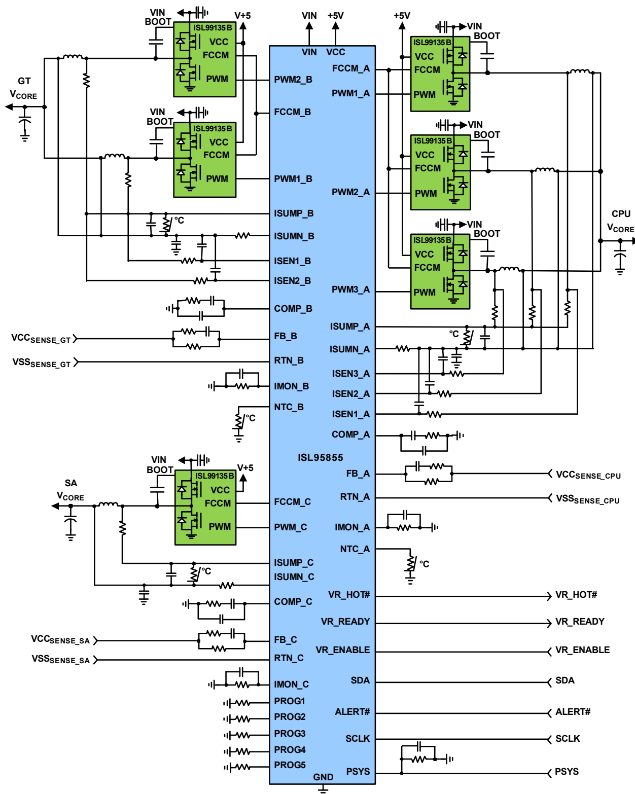
FIGURE 5. TYPICAL APPLICATION CIRCUIT WITH ISL95855
