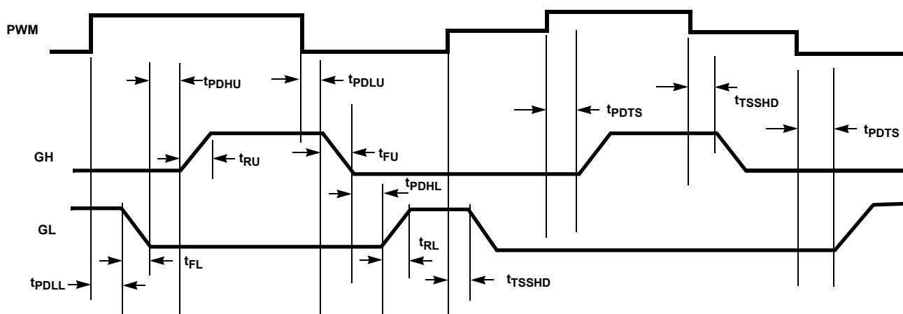
FIGURE 6. TIMING DIAGRAM
