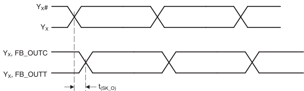
Figure 5. Output Skew
