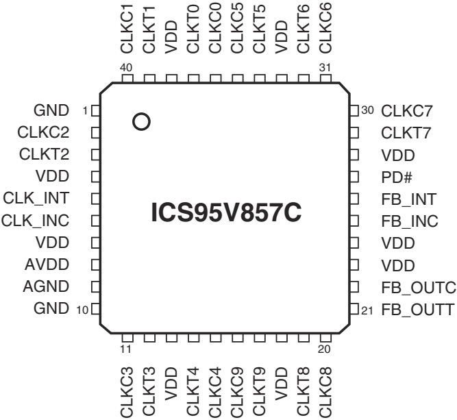
40-Pin MLF
