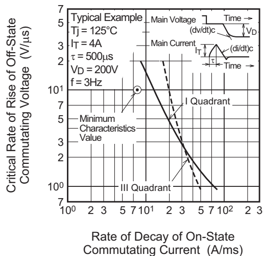
Commutation Characteristics
