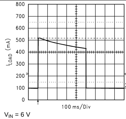
Figure 18. Short-Circuit Current
