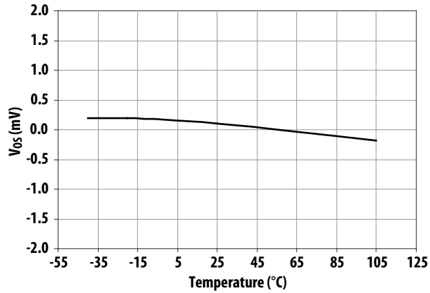
Figure 5. Offset change vs. temperature
