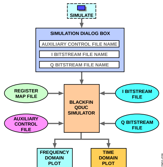
Figure 26. Simulation Block Diagram for QDUC Mode with the Dual Serial Port
