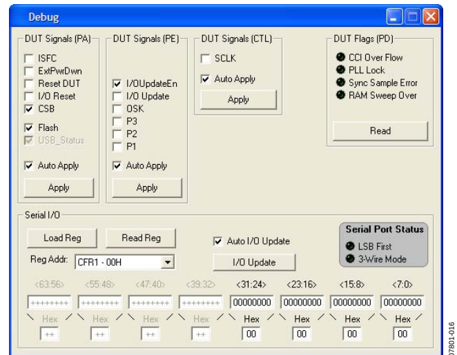
Figure 16. Debug Window
