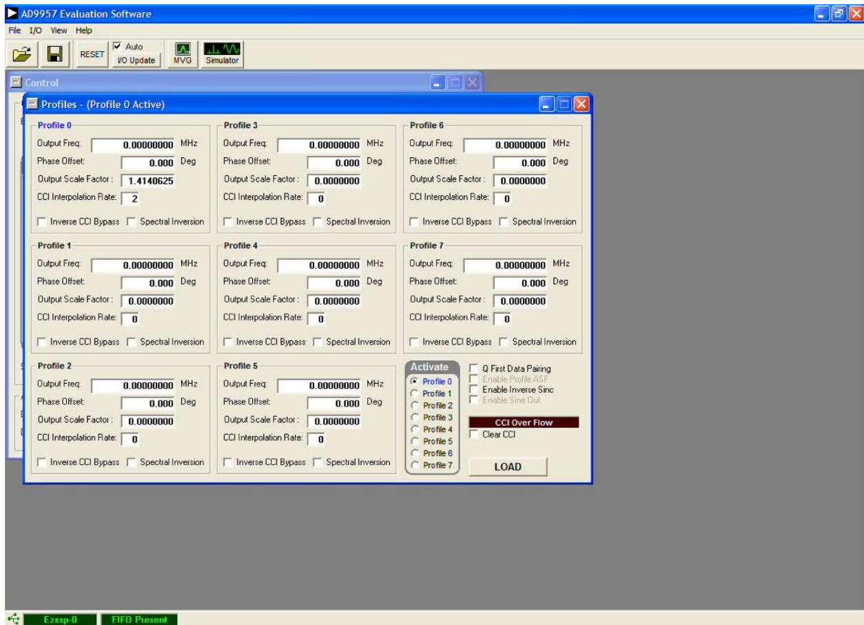
Figure 3. Successful Load
