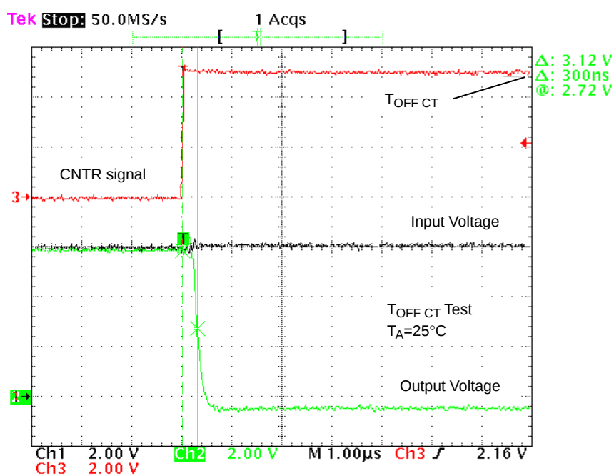
Figure 17. T OFF CT Waveforms
