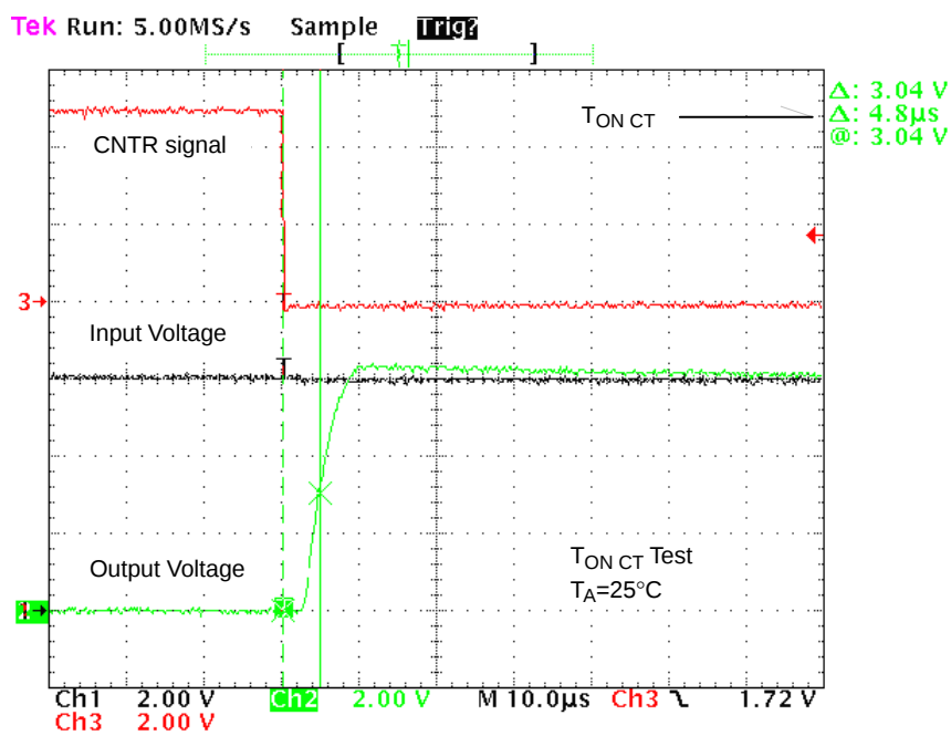
Figure 16. T ON CT Waveforms
