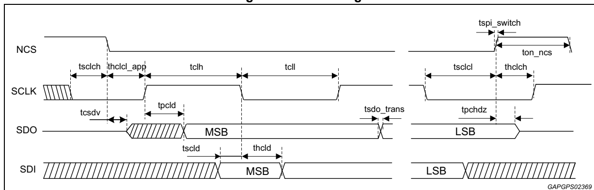
Figure 38. SPI timings
