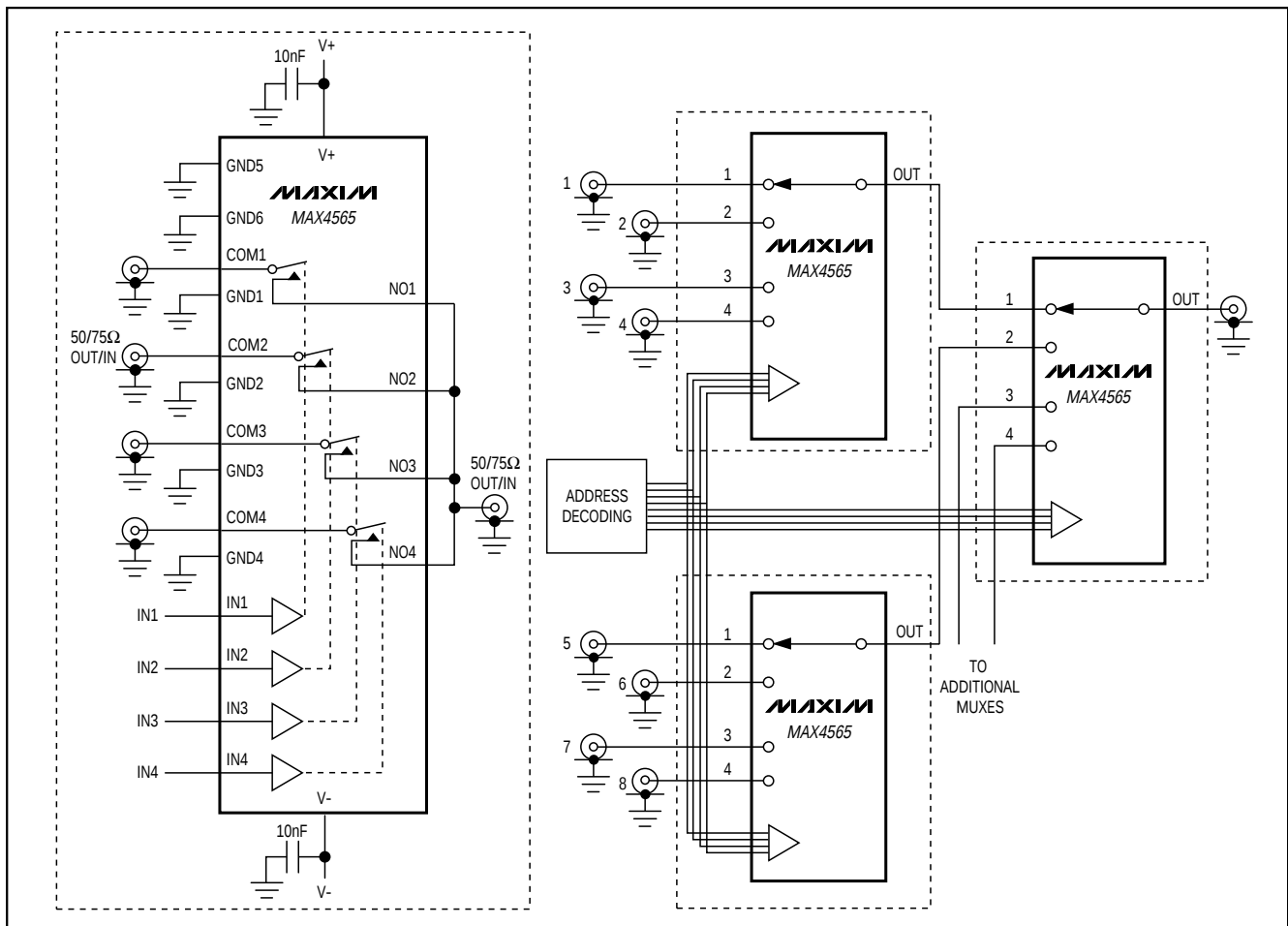
Figure 2. 4-Channel Multiplexer
