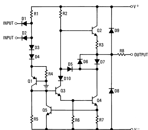
Figure 1. 1/4 Circuit
