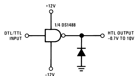
Figure 5. DTL/TTL-to-HTL Translator
