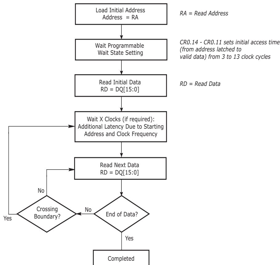
Figure 7.1 Synchronous Read
