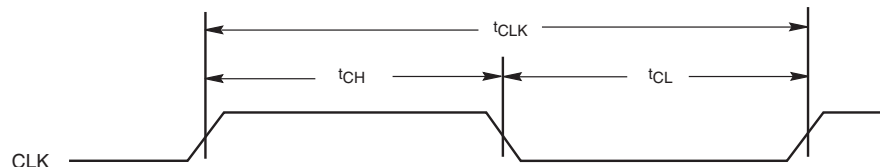
Figure 10.6 CLK Characterization
