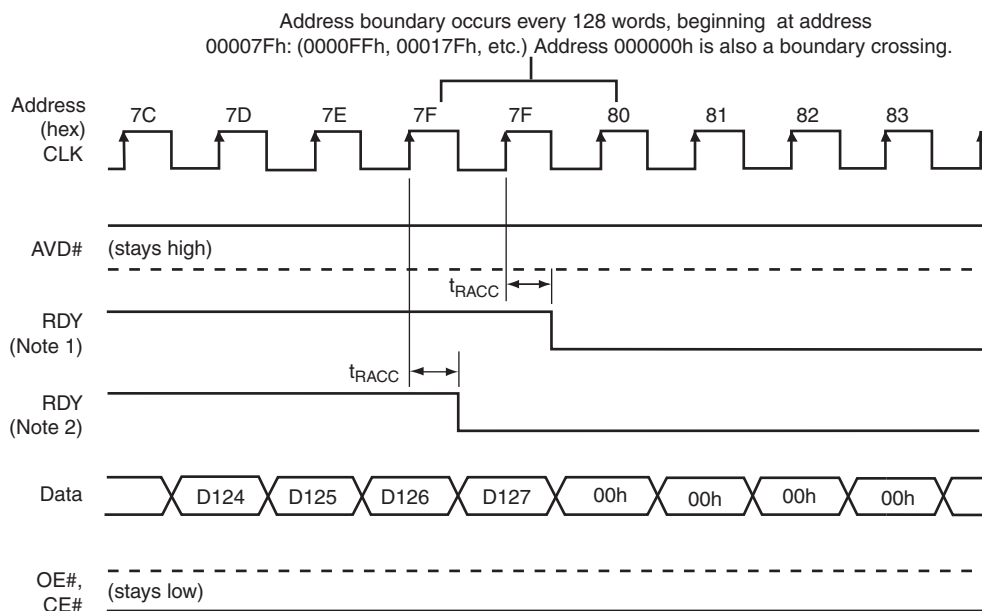
Figure 10.12 Latency with Boundary Crossing into Bank Performing Embedded Operation
