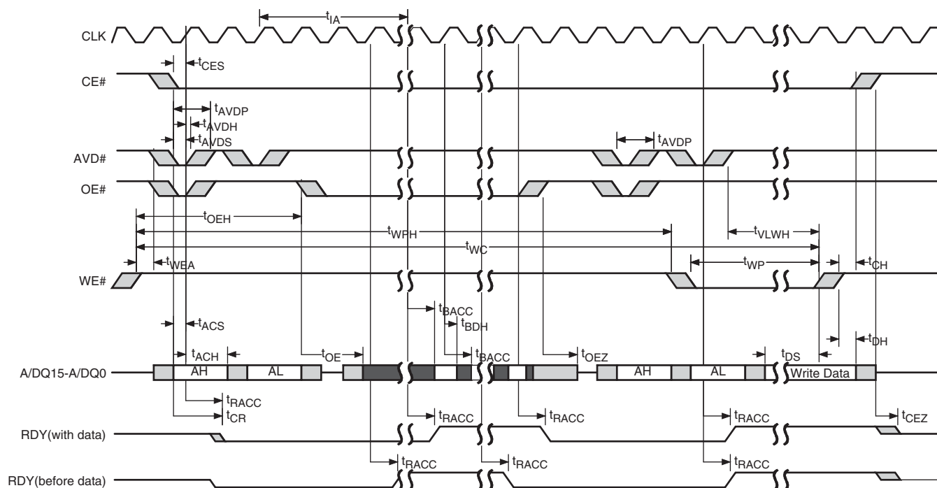
Figure 11.11 Synchronous Read Followed By Write - AADM Interface
