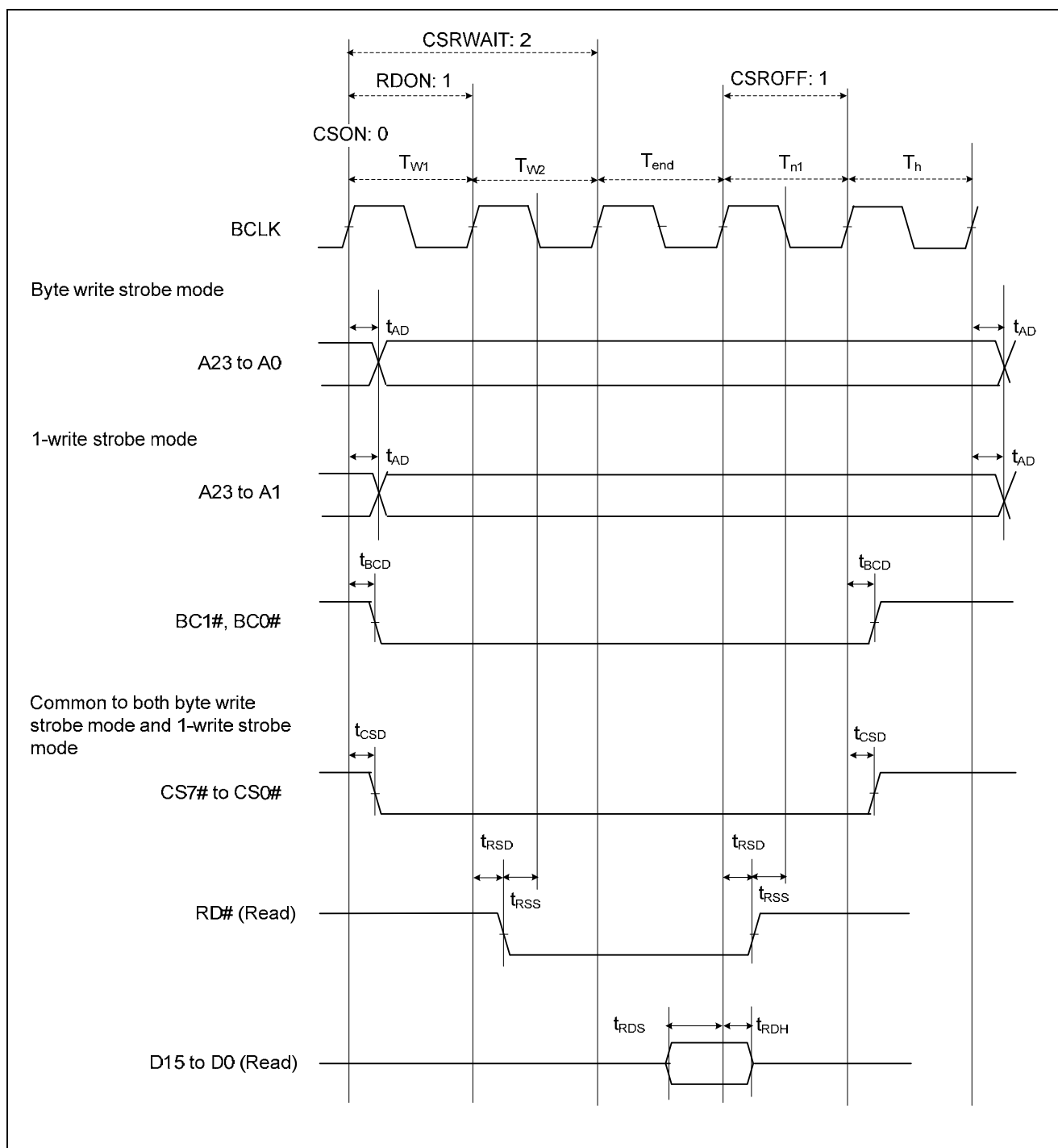
Figure 5.9 External Bus Timing/Normal Read Cycle (Bus Clock Synchronized)
