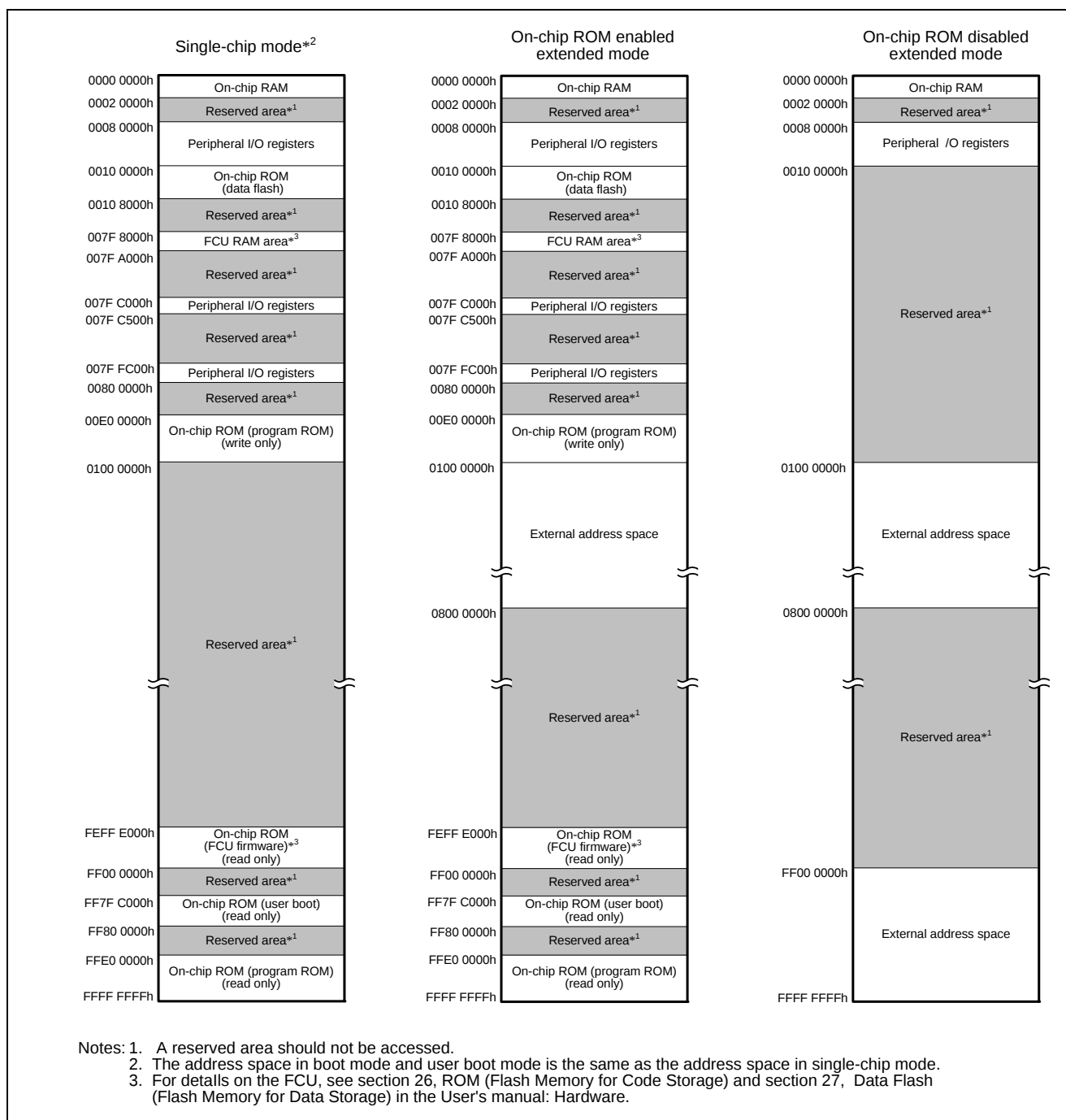
Figure 3.1 Memory Map of the R5F56108
