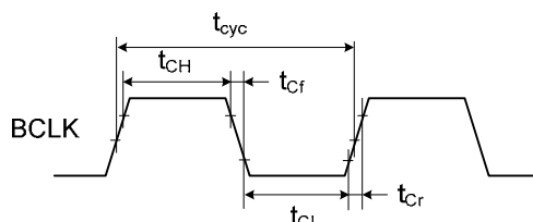
Figure 5.1 External Bus Clock Timing
