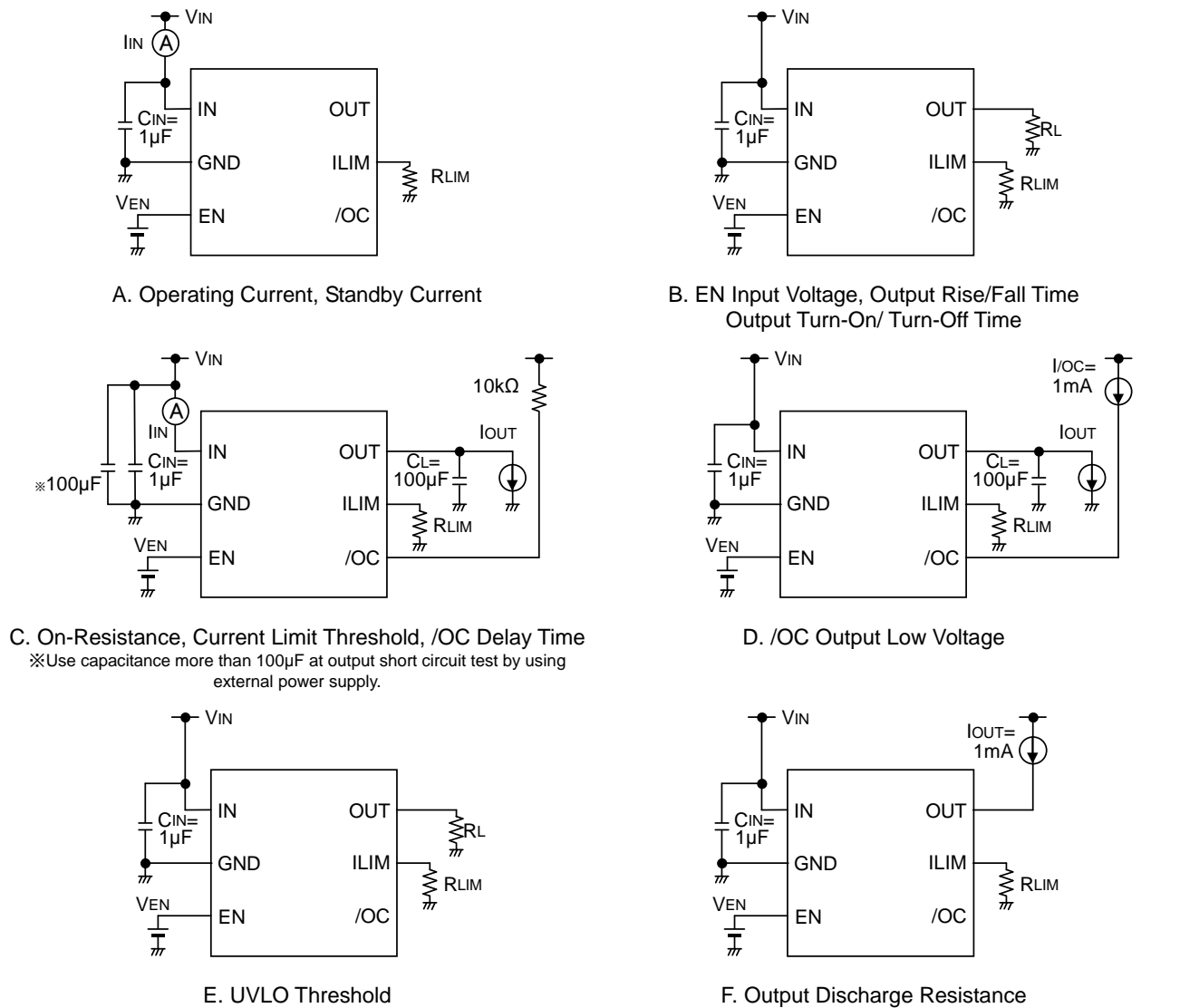
Figure 5. Measurement Circuit
