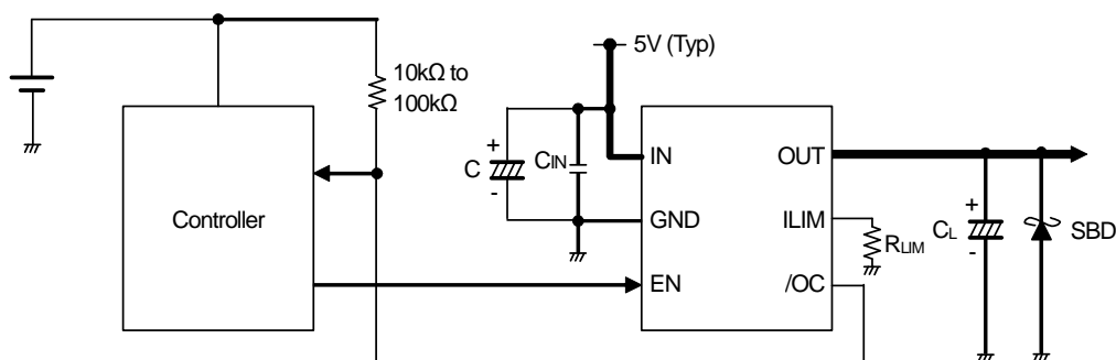
Figure 50. Application Circuit Example
