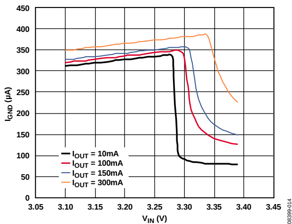
Figure 17. Ground Current vs. Input Voltage (in Dropout)
