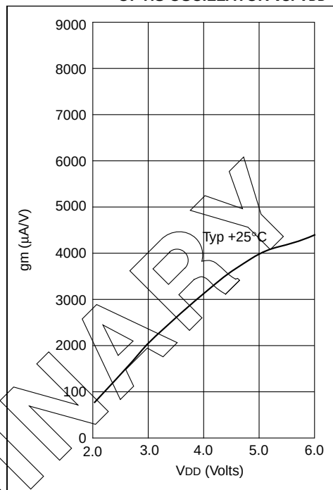
FIGURE 12-14: TRANSCONDUCTANCE (gm) OF HS OSCILLATOR vs. V_{DD}
