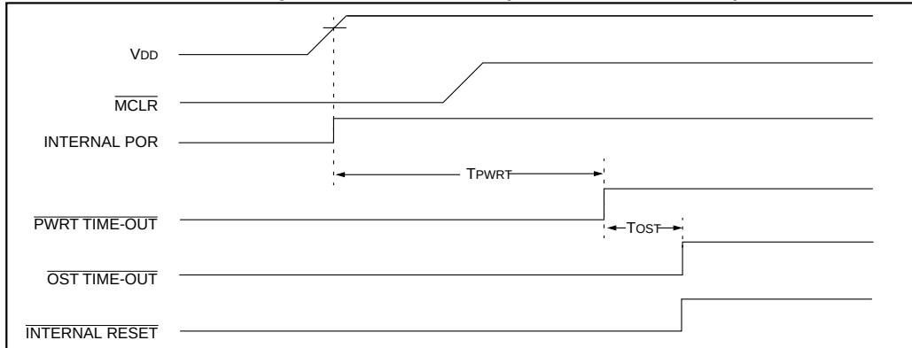
FIGURE 8-11: TIME-OUT SEQUENCE ON POWER-UP ( \overline{\text{MCLR}} NOT TIED TO \text{V}_{\text{DD}} ): CASE 2
