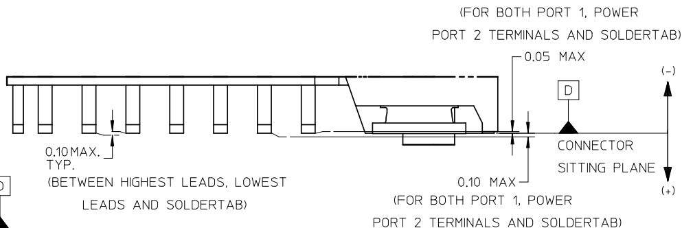
DETAIL 1
