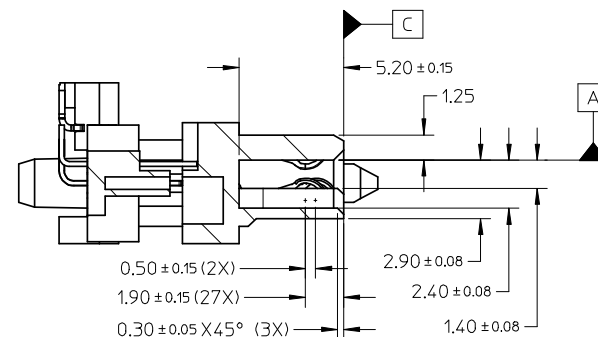
SECTION Z-Z
