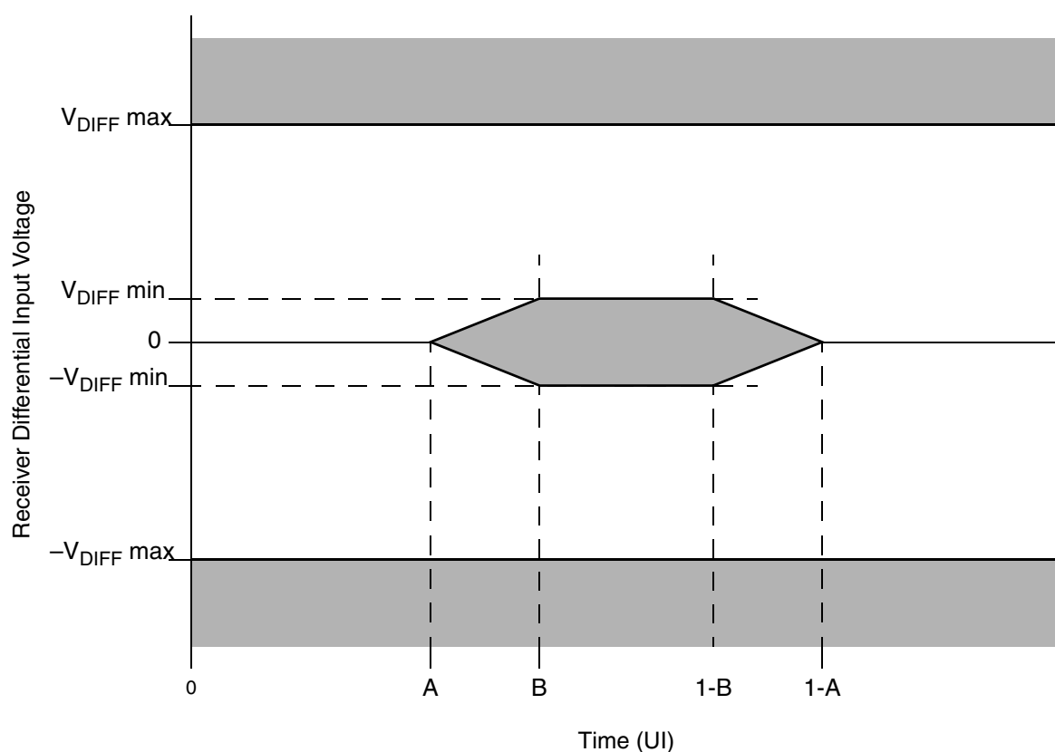
Figure 56. Receiver Input Compliance Mask
