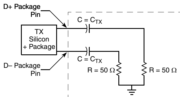
Figure 52. Compliance Test/Measurement Load
