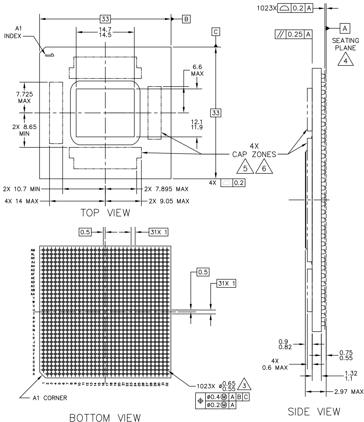
Figure 57. MPC8640D High-Lead FC-CBGA Dimensions
