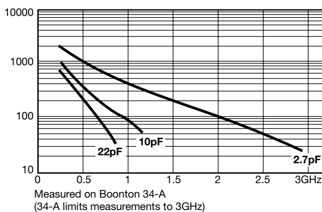
Typical Q vs. Frequency Accu-F®/Accu-P® 0603
