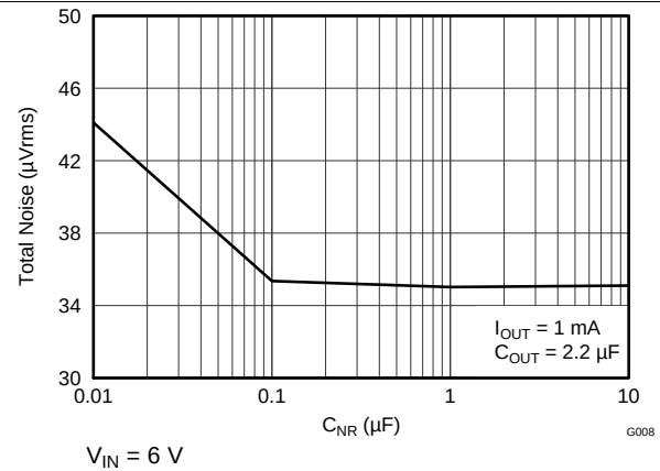
Figure 14. Total Noise vs C_{NR}
