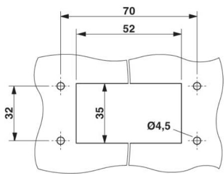
Panel cutout
