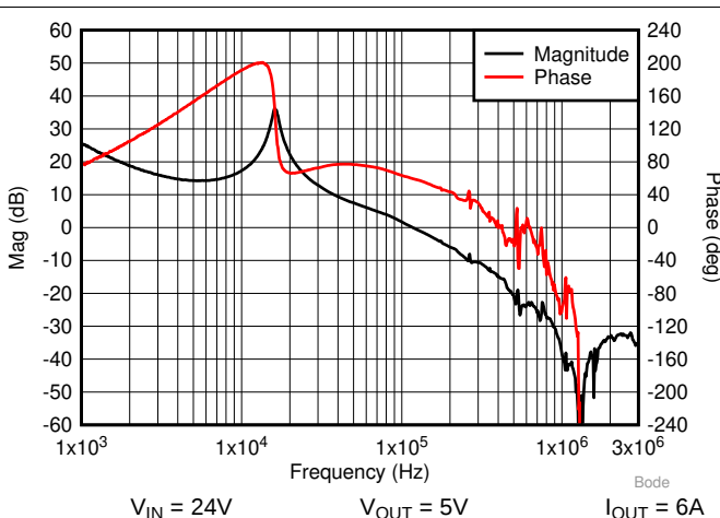
Figure 21. Bode Plot
