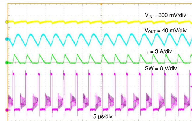
Figure 23. Steady State Waveforms, I_{OUT} = 0.6\text{ A}
