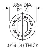
Embossed Aluminum
