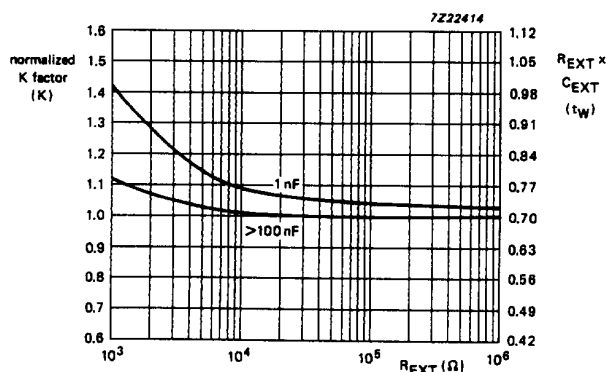
Fig.13 Typical pulse width accuracy versus external resistance; V_{CC} = 4.5 V; T_{amb} = 25 °C.
