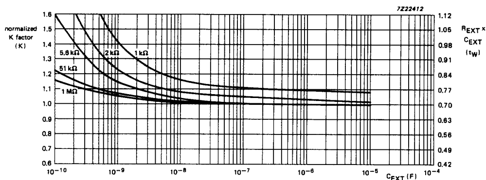
Fig.12 Typical pulse width accuracy versus external capacitance; V_{CC} = 4.5 V; T_{amb} = 25 °C.
