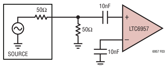
Figure 3. Single-Ended 50\Omega Input Source
