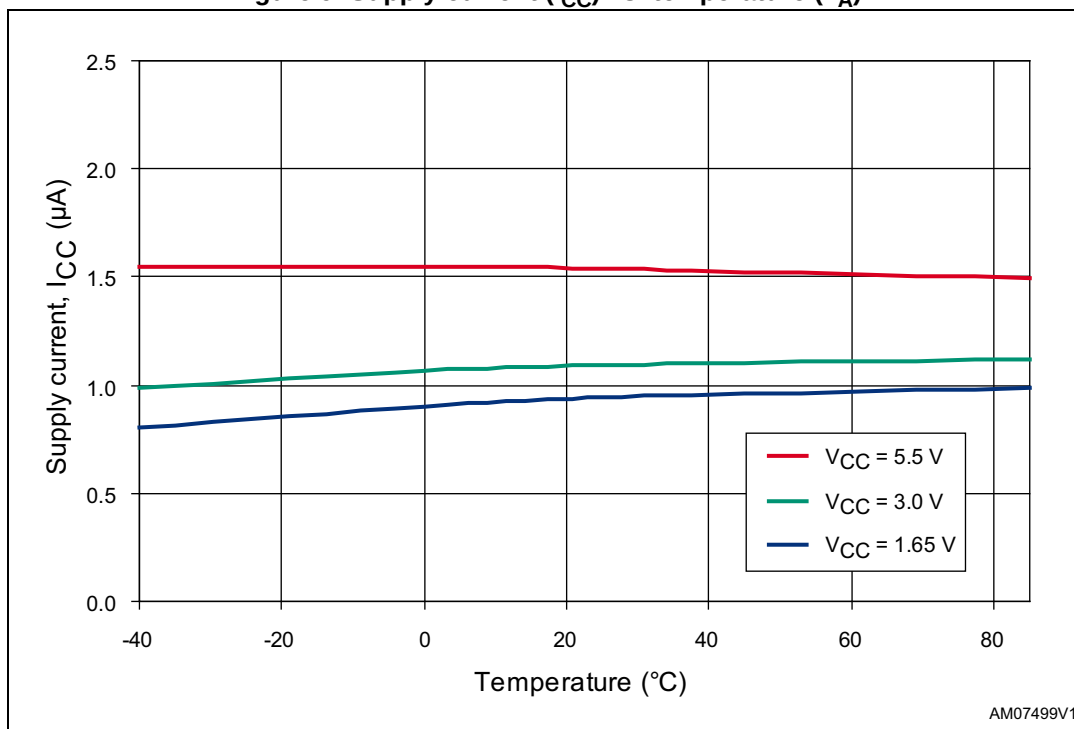
Figure 9. Supply current ( I_{CC} ) vs. temperature ( T_A )
