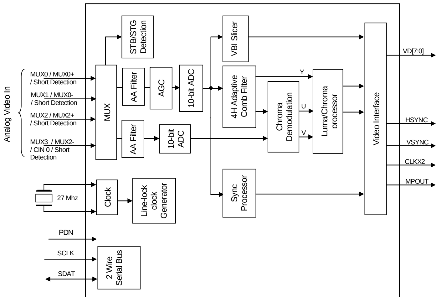
FIGURE 1. TW9990BLOCK DIAGRAM
