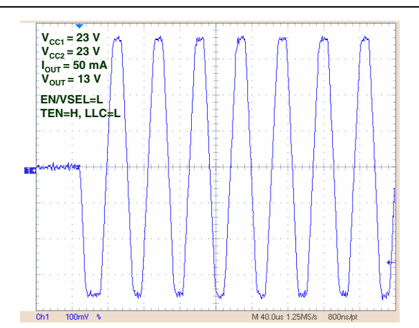
Figure 20. Tone enable
