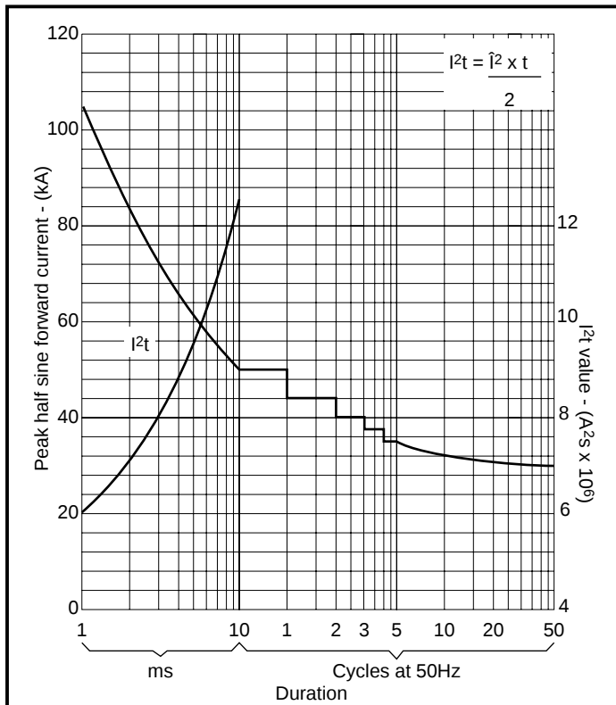
Fig.6 Surge (non-repetitive) forward current vs time (with 50% V_{RRM} at T_{case} 150^\circ C )
