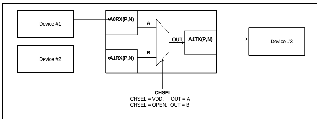
Figure 6 Implementation of Unidirectional 2:1 Mux
