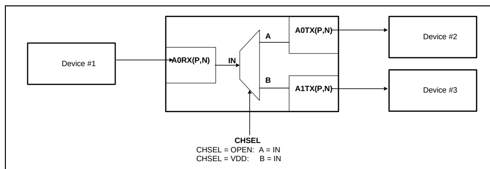
Figure 8 Implementation of Unidirectional 1:2 De-Mux
