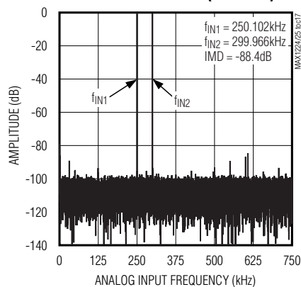
TWO-TONE IMD PLOT (MAX1224)
