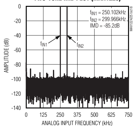
TWO-TONE IMD PLOT (MAX1225)
