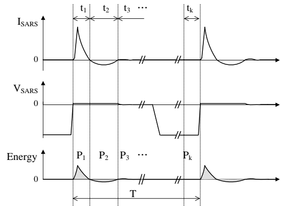
Figure 31. SARS Current
