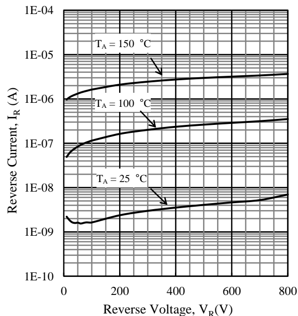
Figure 18. V_R vs. I_R Typical Characteristics
