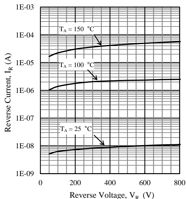
Figure 6. V_R vs. I_R Typical Characteristics
