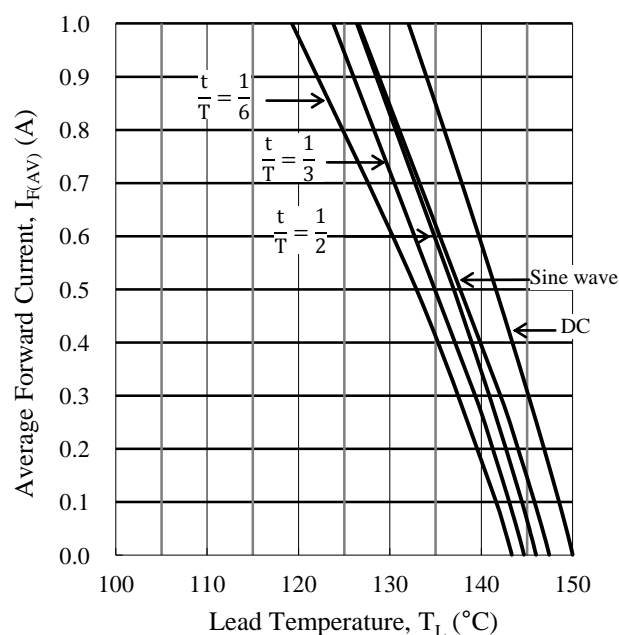
Figure 16. T_L vs. I_{F(AV)} Derating Curves ( V_R = 800\text{ V} , T_J = 150\text{ }^{\circ}\text{C} )
