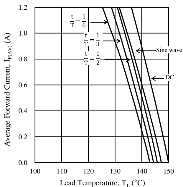
Figure 10. T_L vs. I_{F(AV)} Derating Curves ( V_R = 800 V, T_J = 150 °C)
