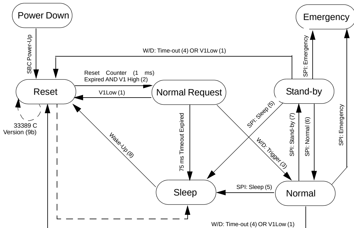
Figure 13. State Machine
