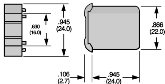
S24SJ (1401, 1403 PUSHWHEEL)
