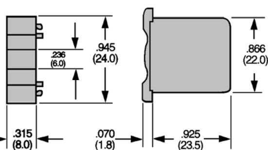
S24SJ (1401, 1403 PUSHWHEEL)
