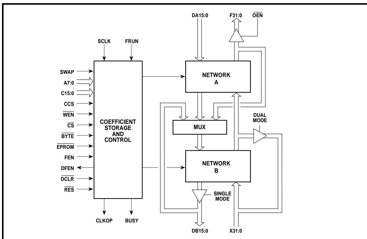
Figure. 4 Block Diagram
