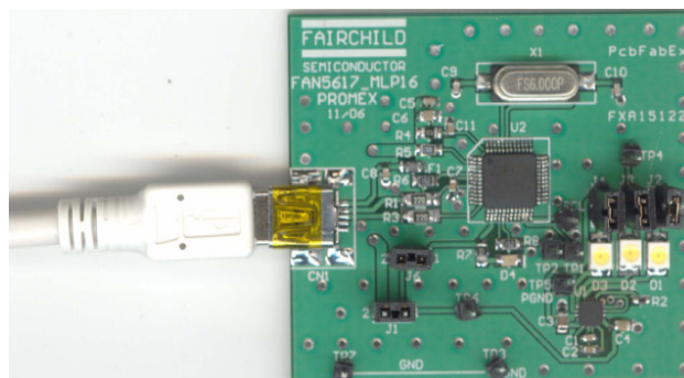
Figure 1: FAN5617MPX Evaluation Board
