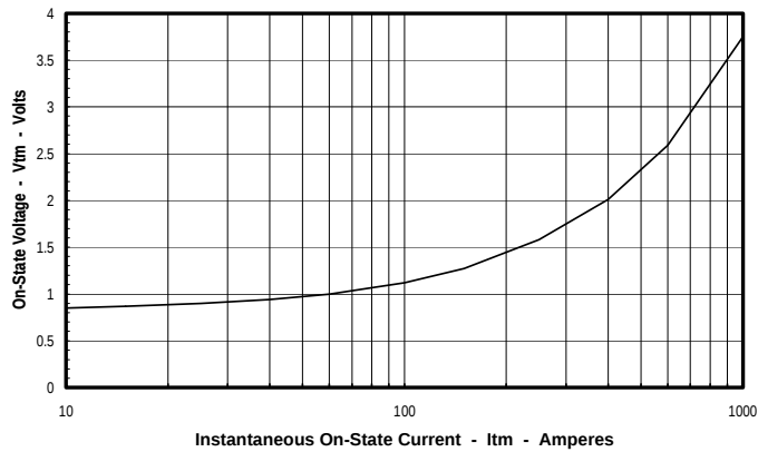
Maximum On-State Forward Voltage Drop ( T_j = 125^\circ\text{C} )
