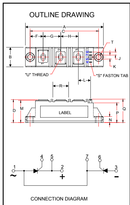
CD43__60A Dual SCR Isolated POW-R-BLOK™ Module 60 Amperes / Up to 1600 Volts
