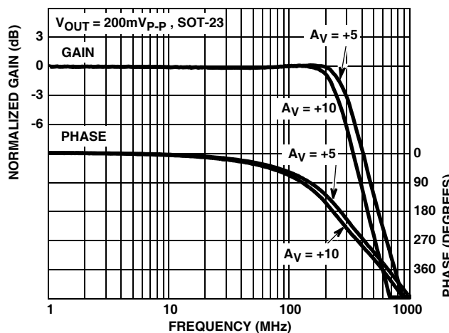
FIGURE 9. FREQUENCY RESPONSE
