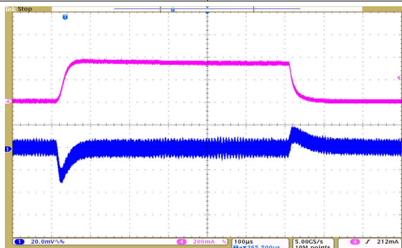
Figure 20. VREG Load Transient Response, 10 mA to 550 mA
