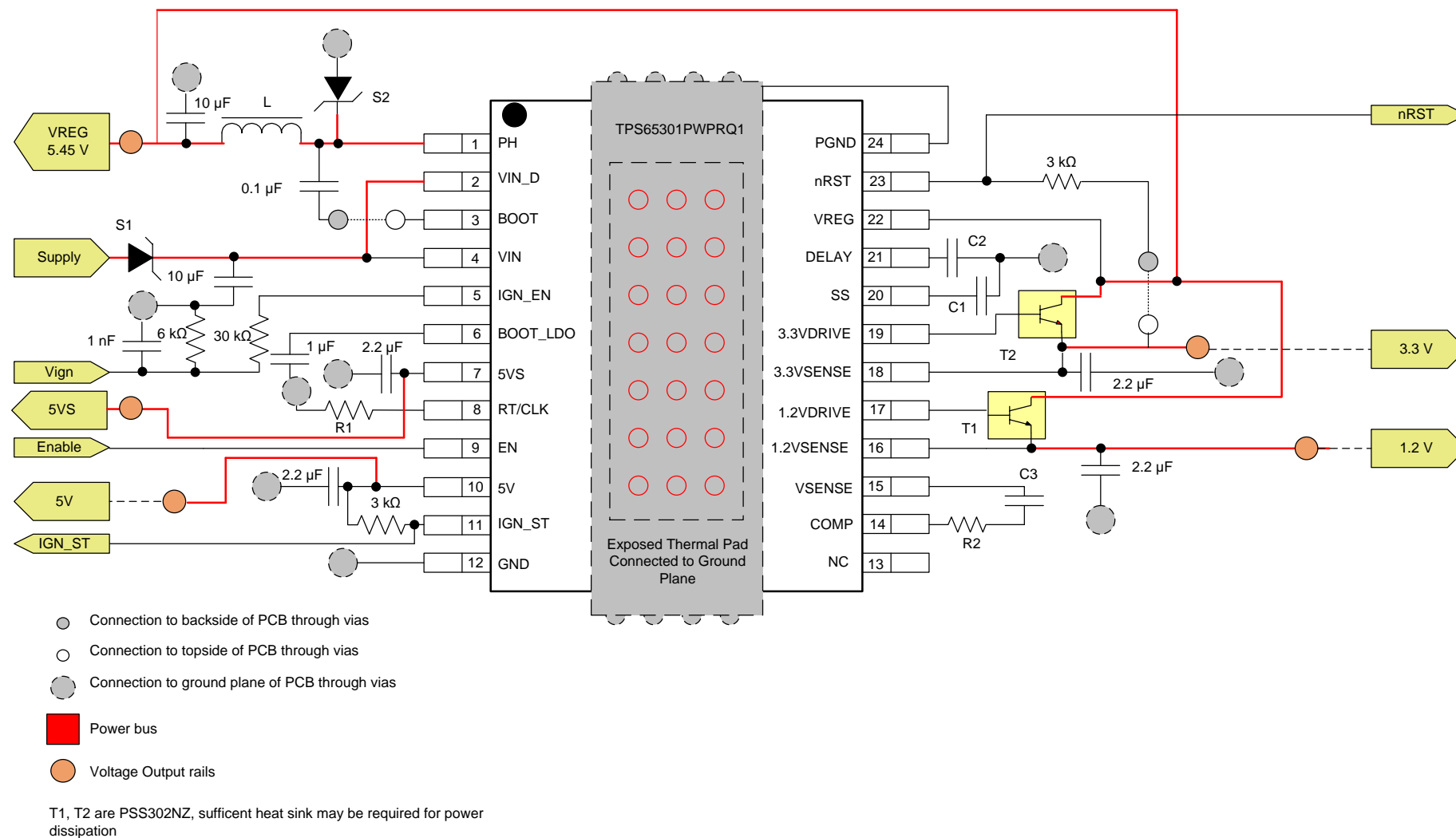
Figure 22. PCB Layout
