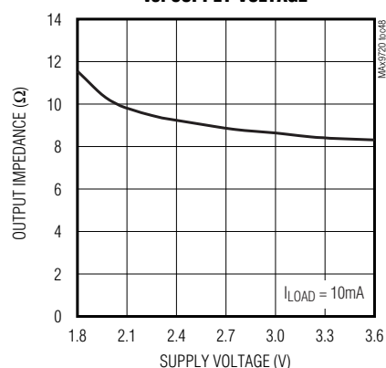
CHARGE-PUMP OUTPUT IMPEDANCE vs. SUPPLY VOLTAGE
