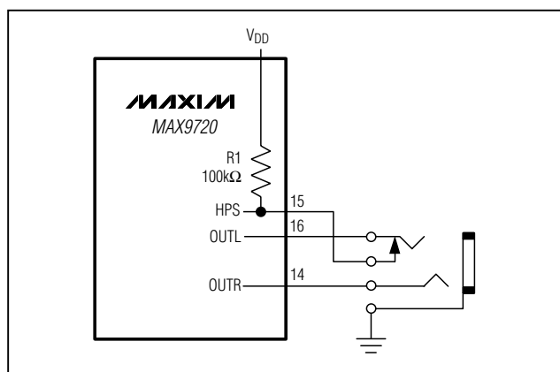
Figure 7. HPS Configuration
