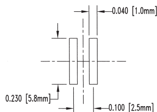
RECOMMENDED FOOTPRINT FOR SM200 AND SM500
