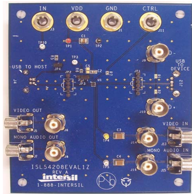
FIGURE 1. ISL54208EVAL1Z EVALUATION BOARD
