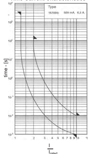
Time-Current Characteristics
