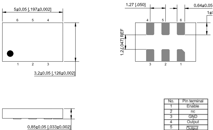
External Dimensions
