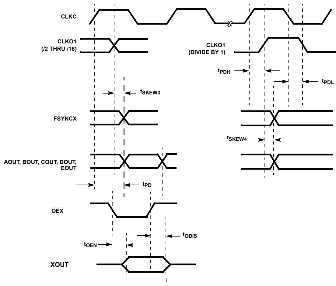
FIGURE 18. OUTPUT TIMING
