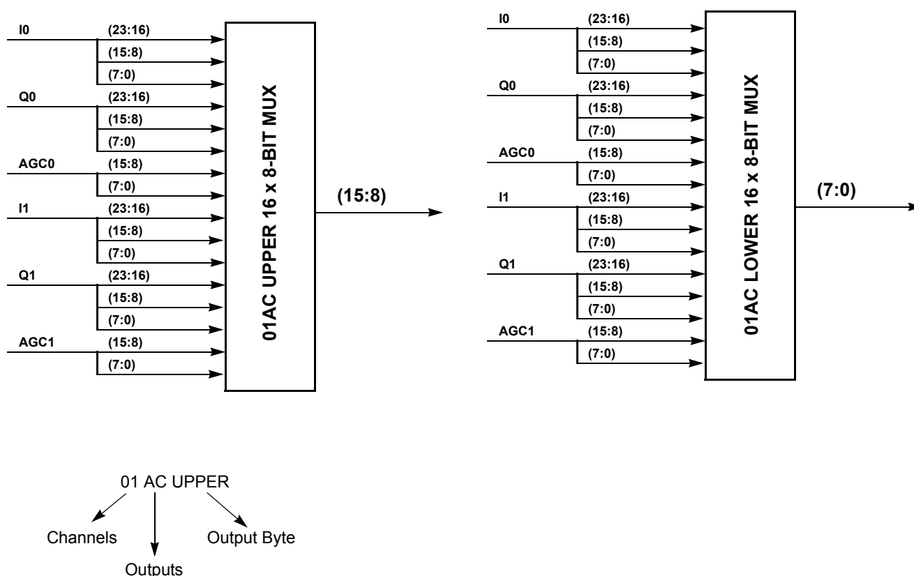
FIGURE 9. MULTIPLEXING CHANNELS
