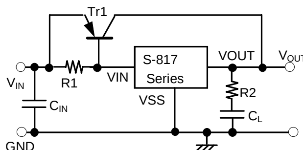
Figure 10 Output Current Boosting
