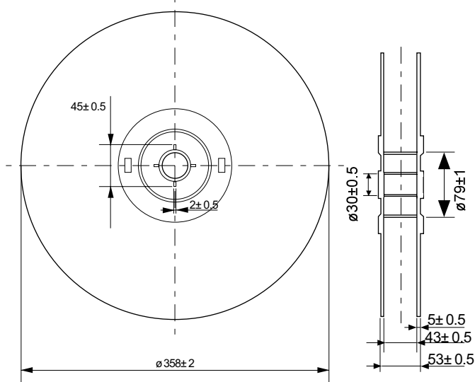
No. YF003-A-R-SD-2.0
