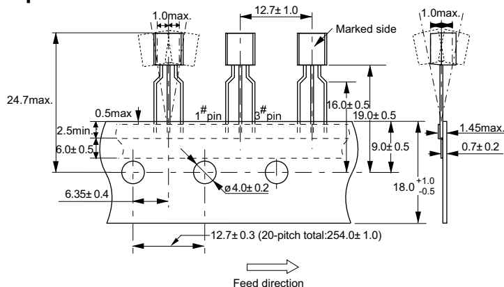
No. YF003-A-R-SD-2.0
