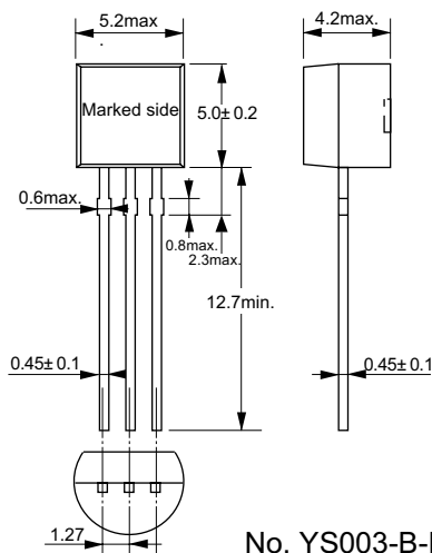
No. YS003-B-P-SD-1.0
