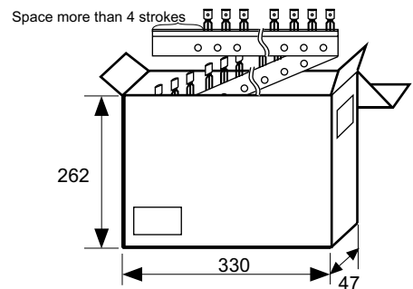
No. YZ003-C-Z-SD-2.0
