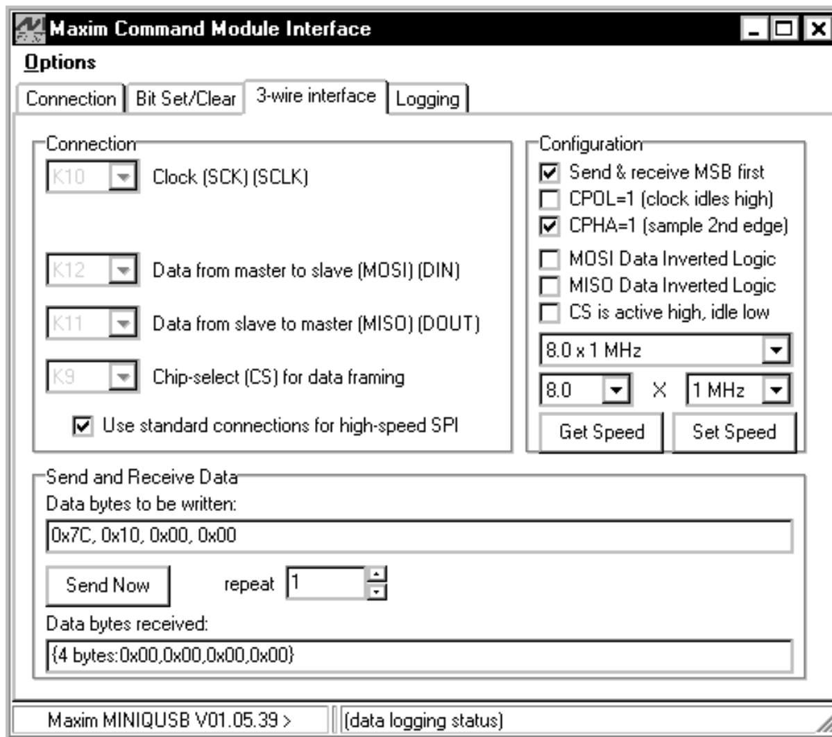
Figure 2. Advanced SPI User Interface Window (3-Wire Interface Tab)
