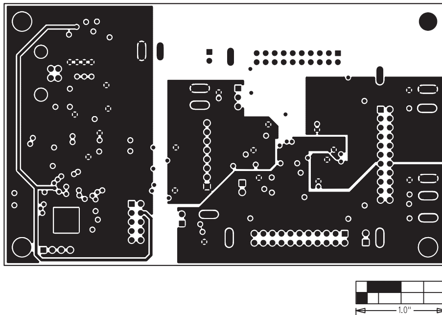
Figure 7. MAX5774 EV Kit PCB—Power Planes (Layer 3)
