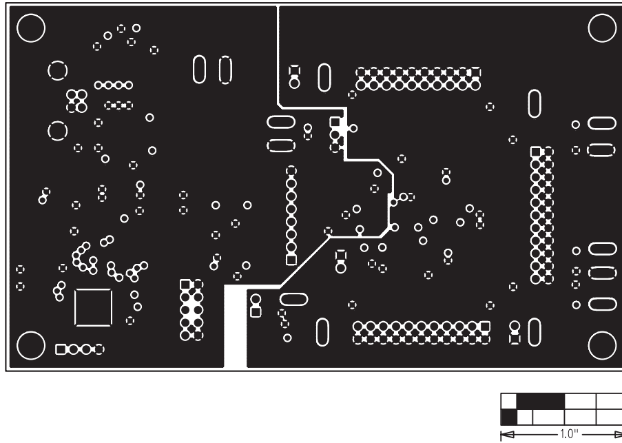
Figure 6. MAX5774 EV Kit PCB—Ground Planes (Layer 2)
