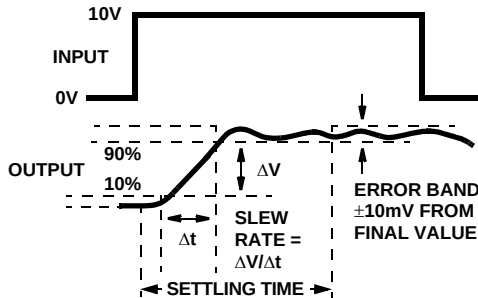
FIGURE 3. SETTLE TIME AND SLEW RATE
