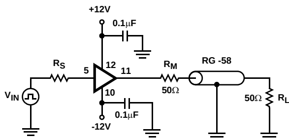
FIGURE 6. VIDEO COAXIAL LINE DRIVER 50Ω SYSTEM
