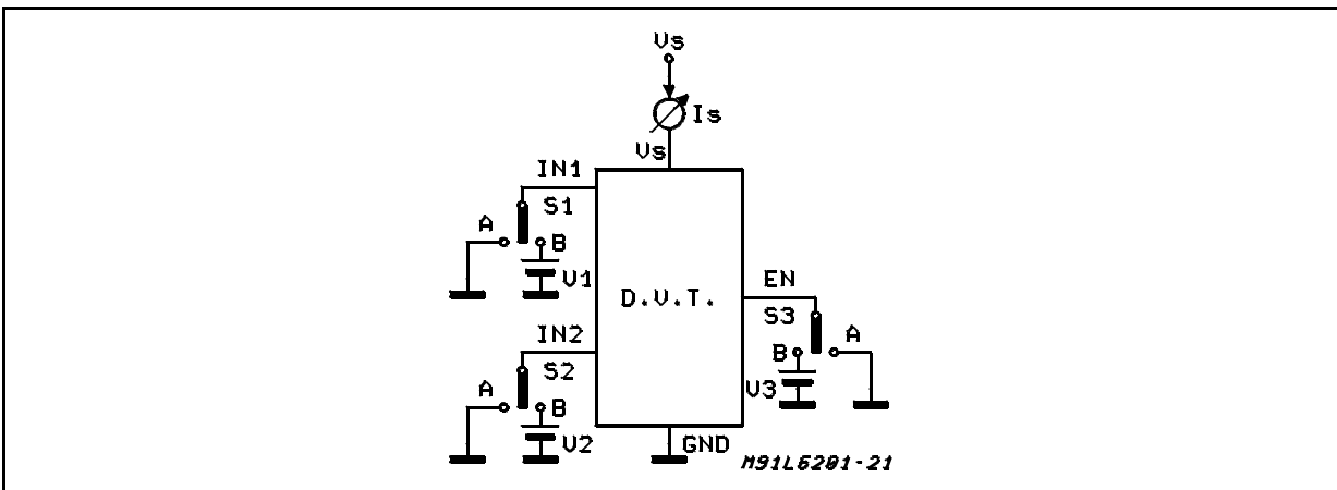
Figure 11: Leakage Current
