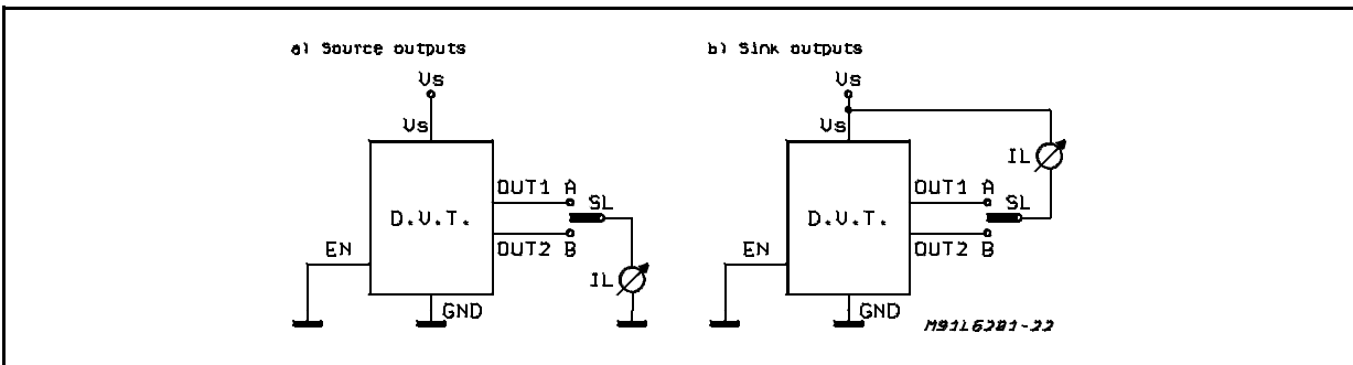
Figure 11: Leakage Current
