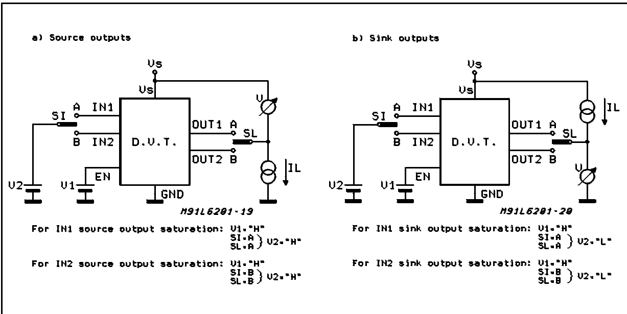
Figure 10: Quiescent Current
